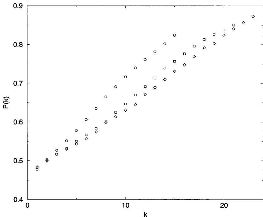
Fig. 7. P(k) versus k , for N=15 (circle), 21 (square), 23 (diamonds) and s=[N/2] . The conditional probabilities have been averaged over a sample of 1000 choices of (\omega_1, \dots, \omega_N) .
