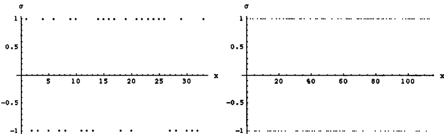
Fig. 1. Ground state for N=33 and N=113 .
