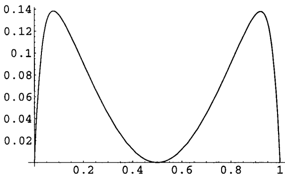
Fig. 6. The function G_1(\lambda) of Eq. (5.67) for \lambda \in [0, 1] .
