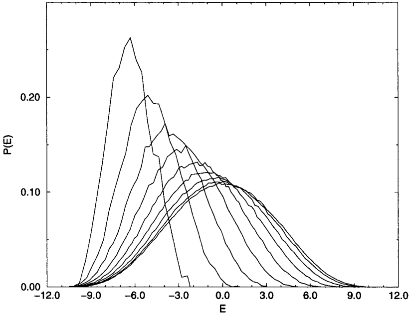
Fig. 3. Distributions of the energy over the subspaces \Omega_s . The size of the system is N = 23 and s = 3, 4, \dots, 11 from left to right. The cases s = 1 and s = 2 behave in a similar way, but they are not plotted because of the small number of sample points for this lattice size N .
