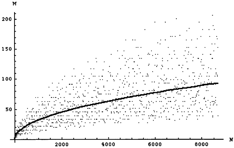
Fig. 2. Total magnetization Nm^0 of the ground state versus N , 2N+1=4m+3 prime. The continuous curve is \sqrt{N} .
