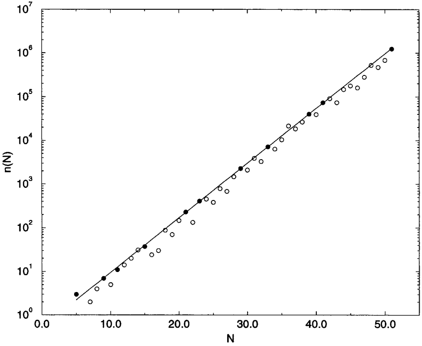
Fig. 4. The number of metastable states n(N) for N . The line represents the best fit n(N) \approx e^{\lambda N} with \lambda \approx 0.28 for values of N such that p = 2N + 1 is a prime of the form 4m + 3 (filled points). Other points are for generic integer N .
