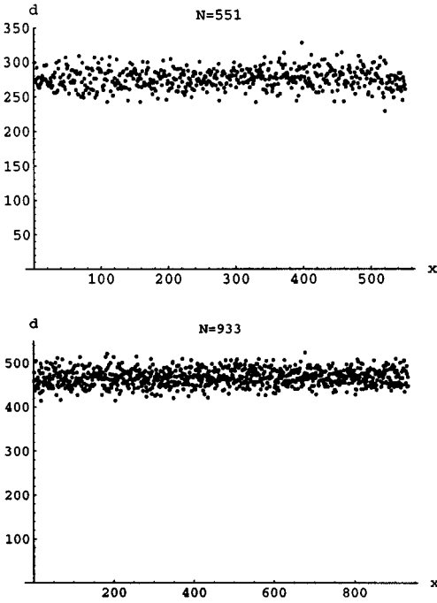
Fig. 9. The function d_N(x) versus x , for N = 551 and N = 933 .
