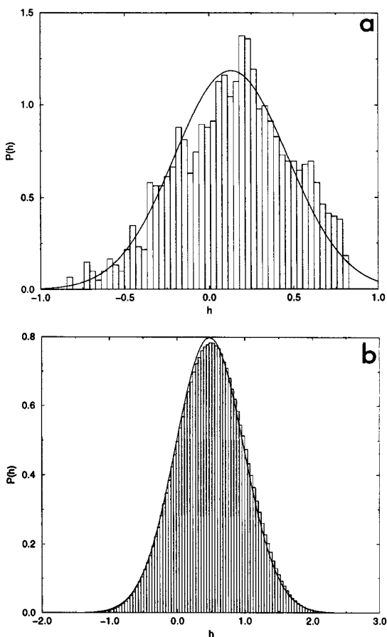
Fig. 5. Distribution of the function h(\tau, \omega) for a fixed \omega \in \{1, \dots, N\} and \tau varying in \Omega_s . Here N = 23 and s = 3 (a) and s = 11 (b). The solid line is the gaussian distribution in the r.h.s. of (5.50).
