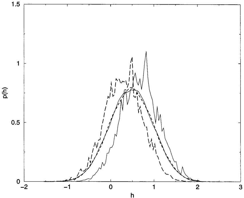
Fig. 8. Graphs of the four distributions of the values of h described in the text.
